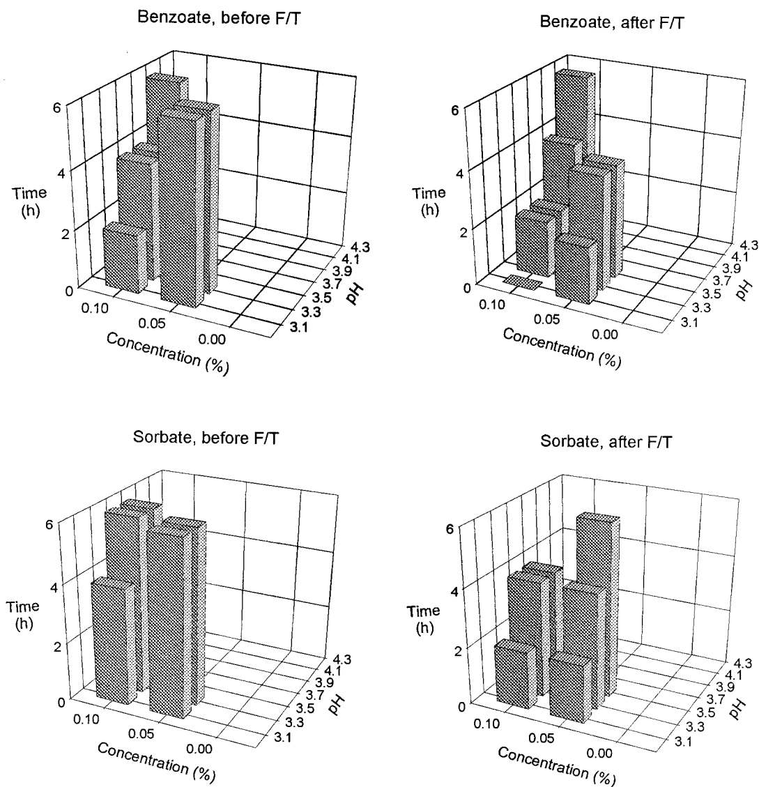
FIG. 2. Effects of storage time, preservative concentration, and pH on achieving a 5-log 10 -unit reduction in E. coli O157:H7 populations in apple cider at 35°C before and after an F-T treatment. The height of a given bar indicates the time, for a given preservative concentration and pH, at which the observed probability of achieving a 5-log 10 -unit reduction was at least 0.5. A bar with no height indicates 0 h, and no bar present indicates >6 h for a given preservative concentration and pH at which the observed probability of achieving a \geq 5 -log 10 -unit reduction was at least 0.5.
