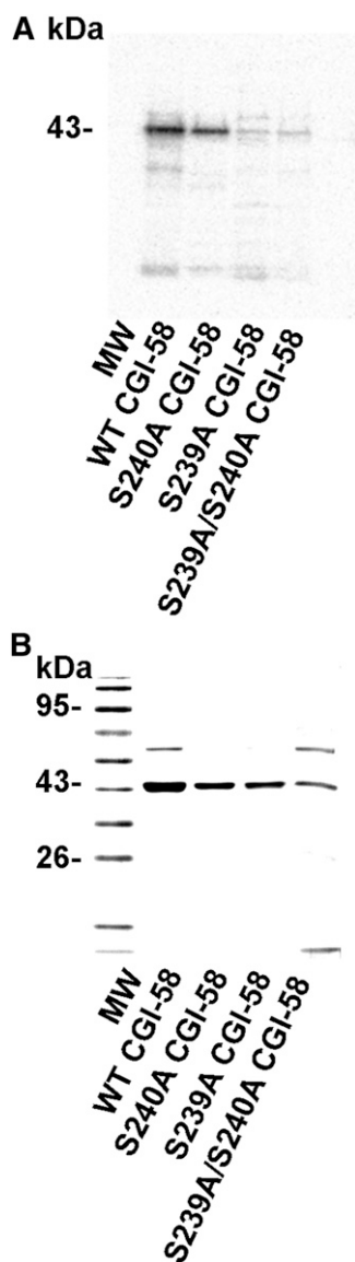
Fig. 3. CGI-58 is phosphorylated in vitro by PKA on Ser239. Recombinant CGI-58 (WT) or S240A-, S239A-, or S239A/S240A-mutated CGI-58 (1 μg) were incubated with PKA (0.32 unit/ml) and 50 μM [ \gamma - ^{32} P]ATP before SDS-PAGE, transfer to PVDF, and phosphorimaging analysis (A). B: Coomassie-stained gel prior to protein transfer.
